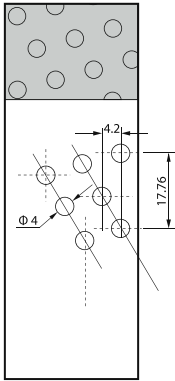
圆形油孔内孔 > Φ 25 Spherical Holes Inter Diameter > Φ 25
